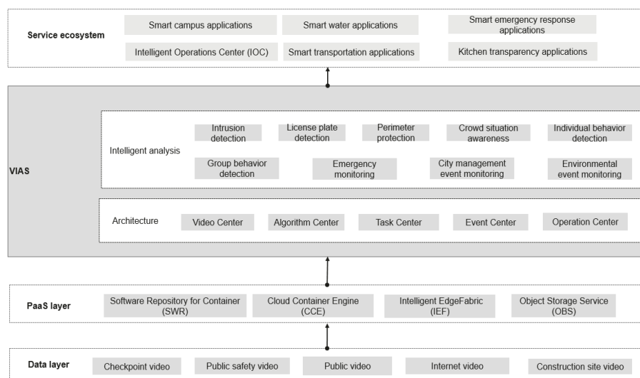
Figure 1-1 Solution architecture
